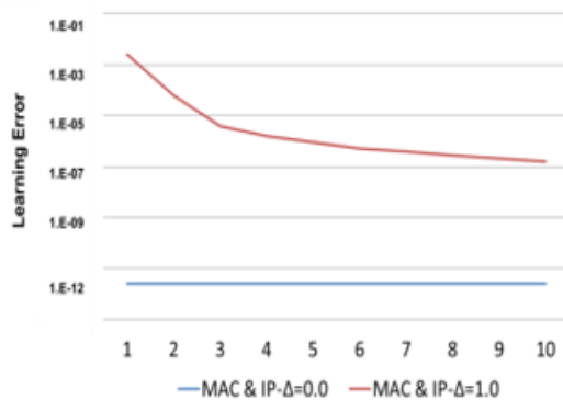
Fig.3. Changes in \Delta with respect to MAC & IP
