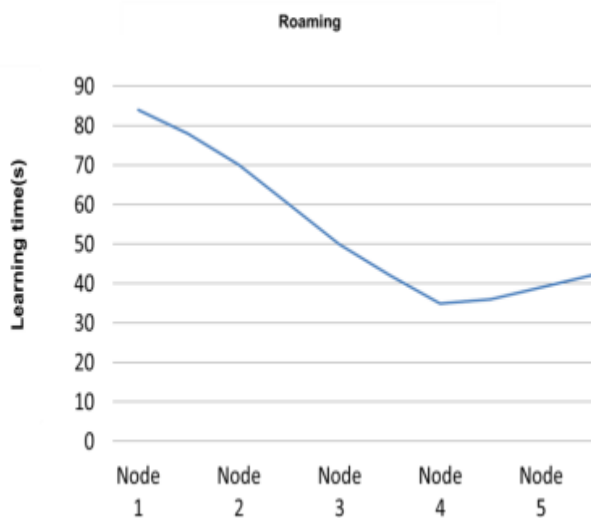
Fig.4 Learning and Mining Iterations in 5G network simulation
